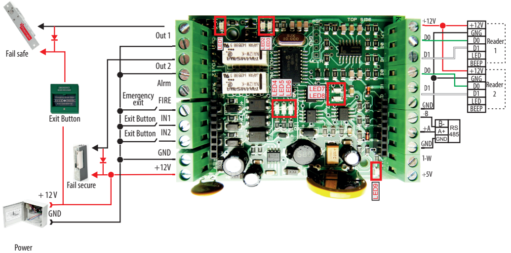
Wiring Diagram LED and BEEP
