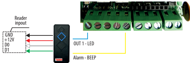
Wiring Diagram LED and BEEP
